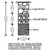
SECTION OF RAIN WATER COLLECTION PITS (NTS)
