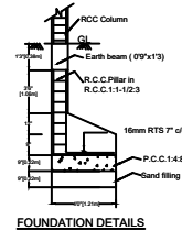
FOUNDATION DETAILS
