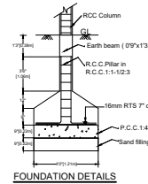
FOUNDATION DETAILS
