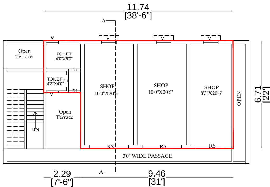
PRO.,FIRST FLOOR PLAN
