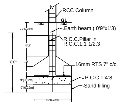
FOUNDATION DETAILS
