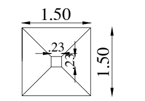
COLUMN FOUNDATION
