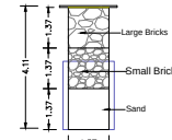
SECTION OF RAIN WATER COLLECTION PITS (NTS)
