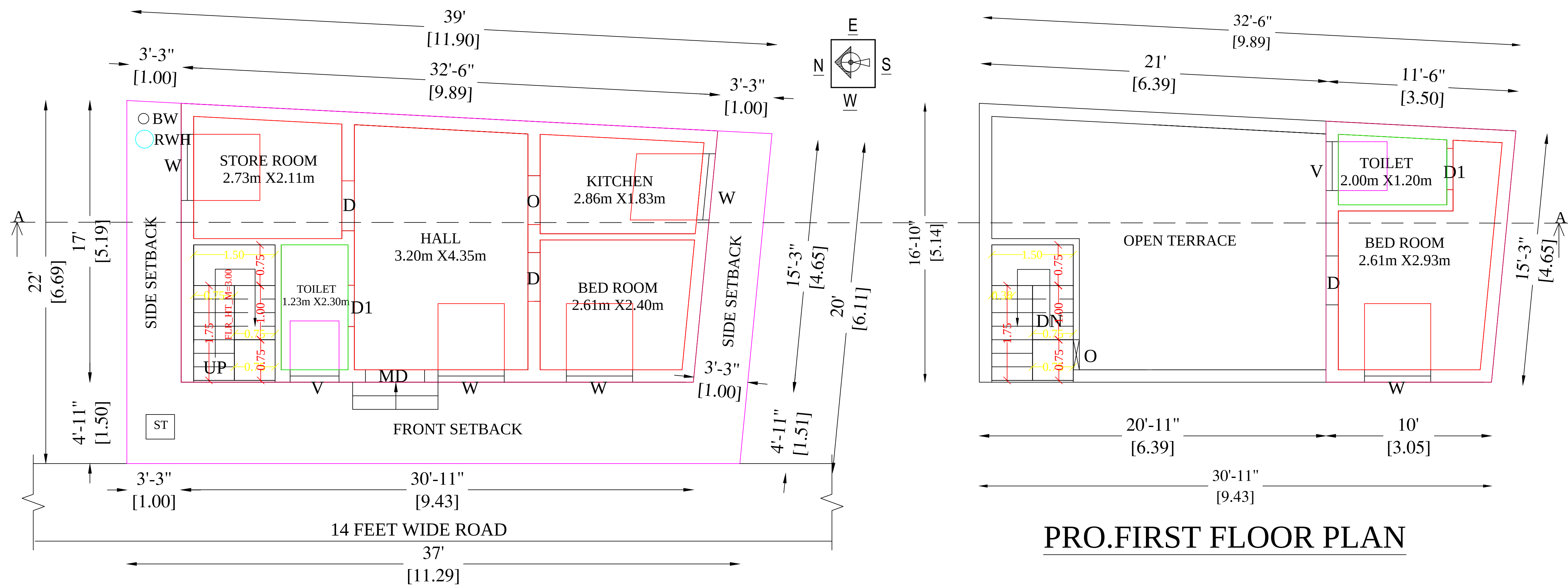
PRO.GROUND FLOOR PLAN
