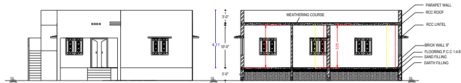
Section on A-B
