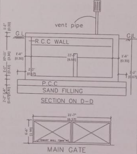
SECTION ON D-D
