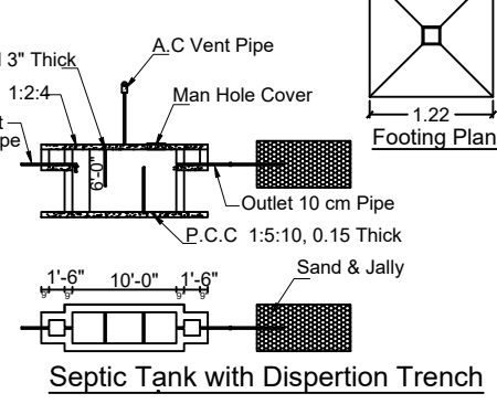
Septic Tank with Dispersion Trench
