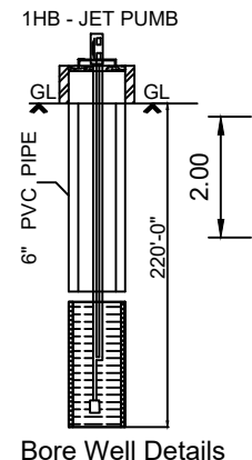
Bore Well Details
