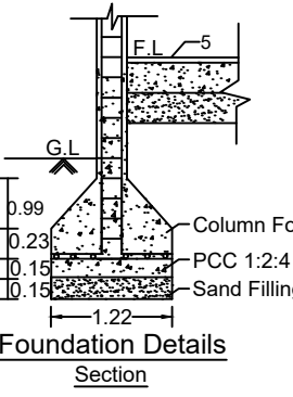
Foundation Details
