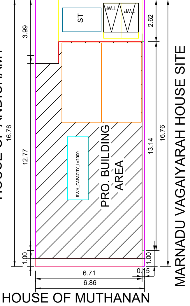
SITE PLAN
