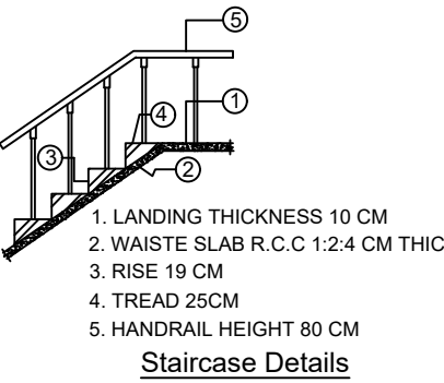
Staircase Details
