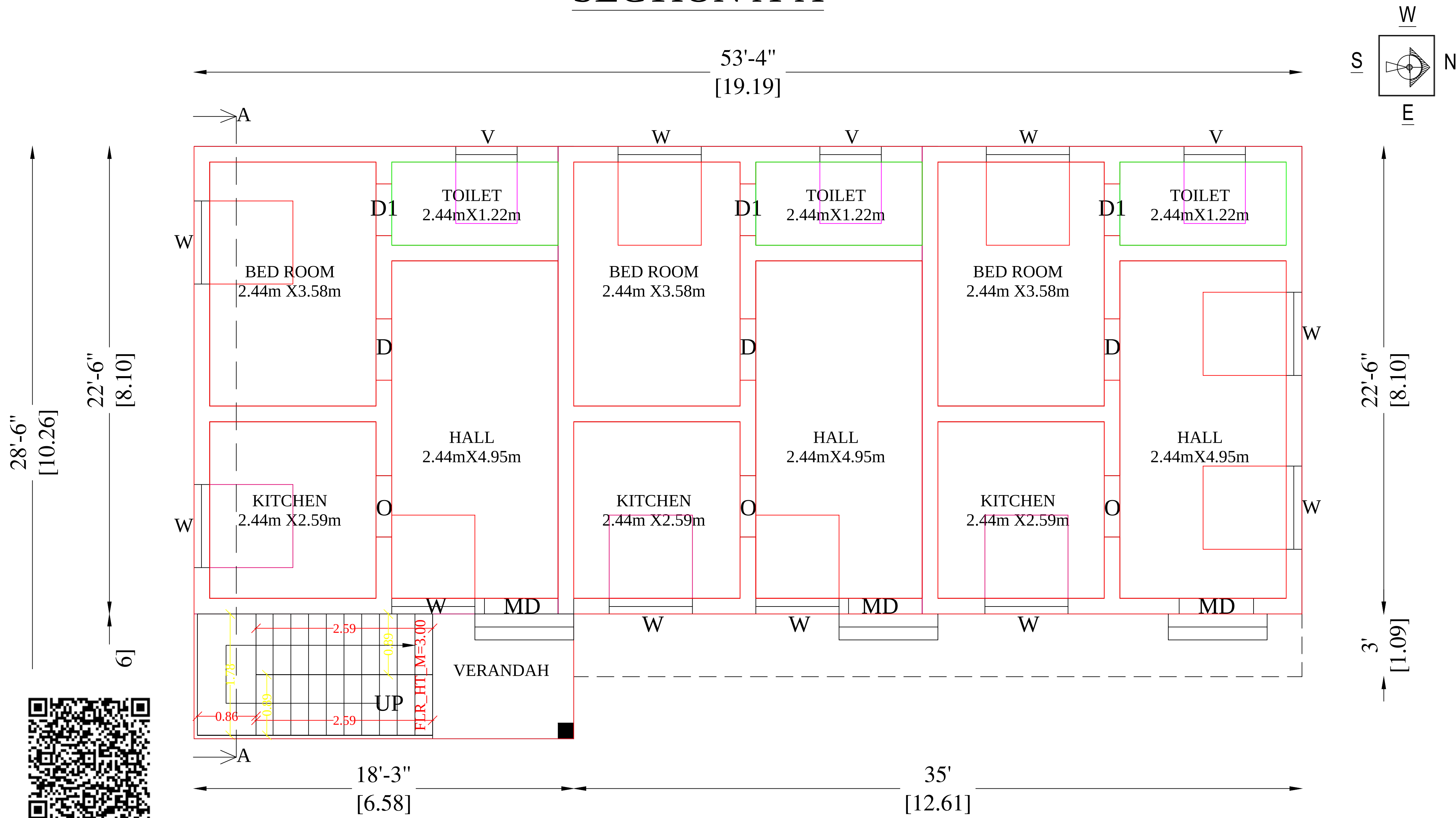
PRO. GROUND FLOOR PLAN
