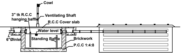
SECTION DETAILS OF SEPTIC TANK
