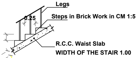
STAIRCASE DETAILS
