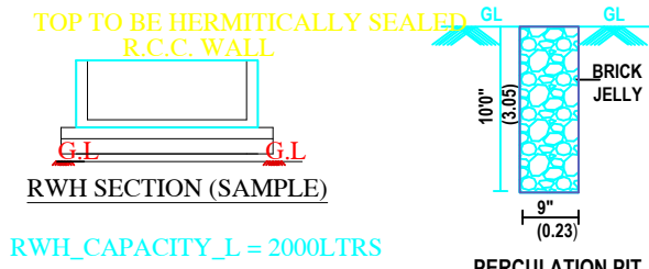
RW H SECTION (SAMPLE)
