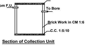
Section of Collection Unit
