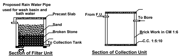
Section of Filter Unit
