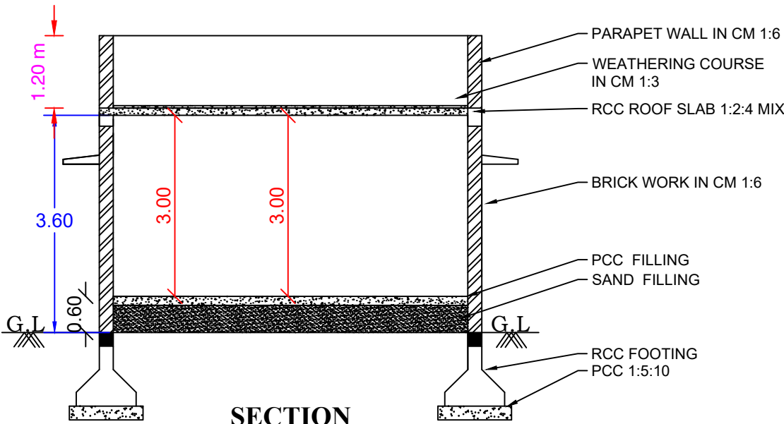
SECTION
