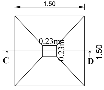
SECTION - 'CD'
