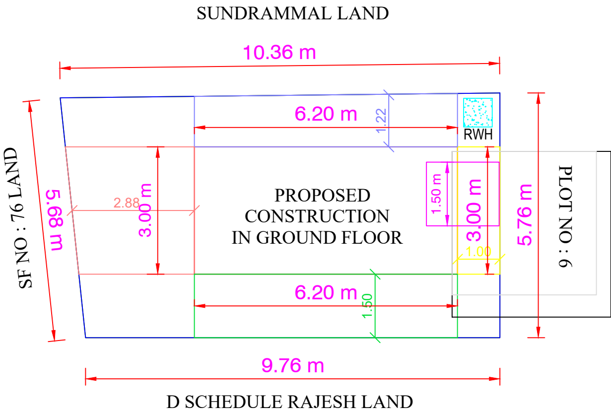
SITE PLAN
