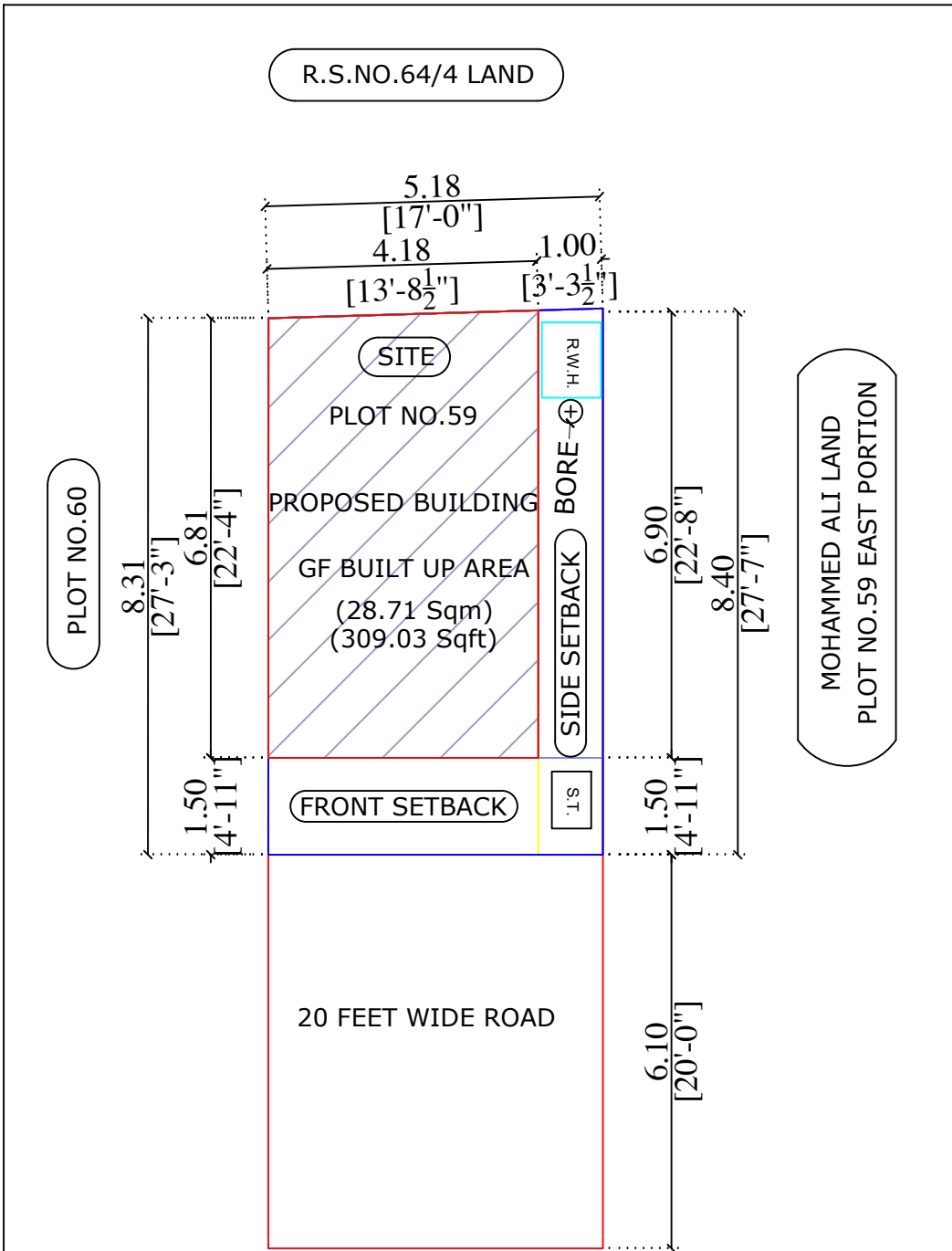
SITE PLAN
