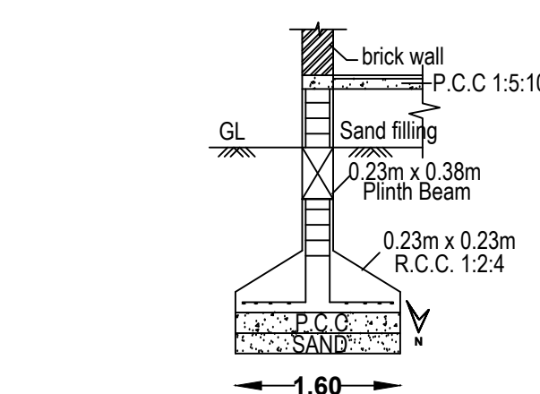
1.60 FOUNDATION DETAILS
