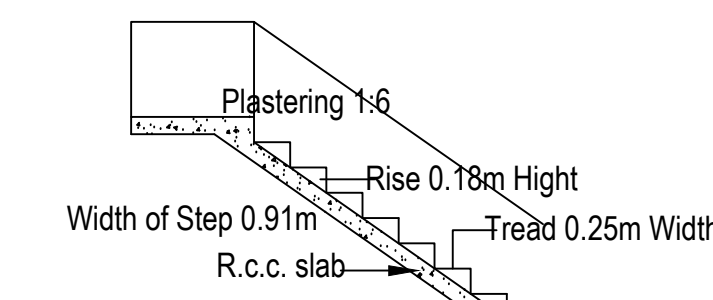
DETAILS OF STAIR CASE
