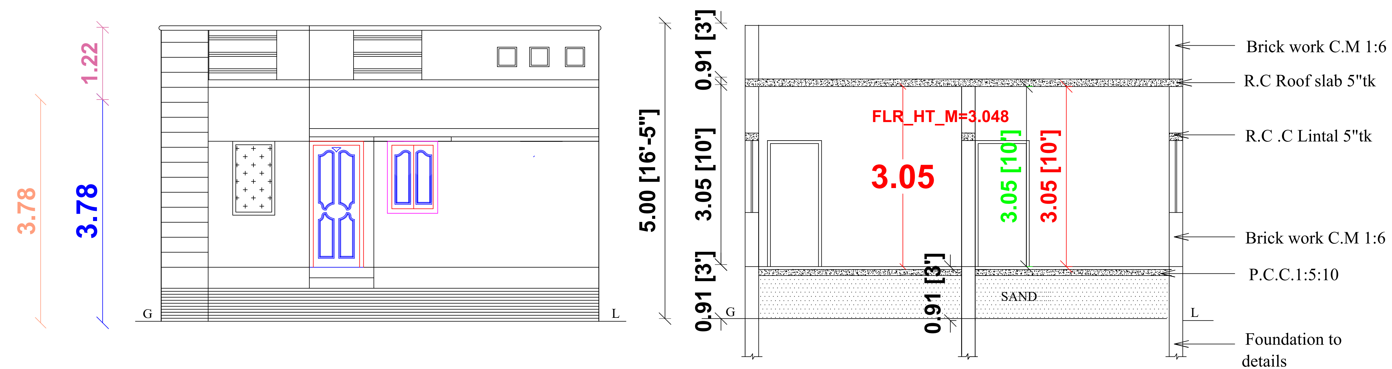
FRONT ELEVATION
