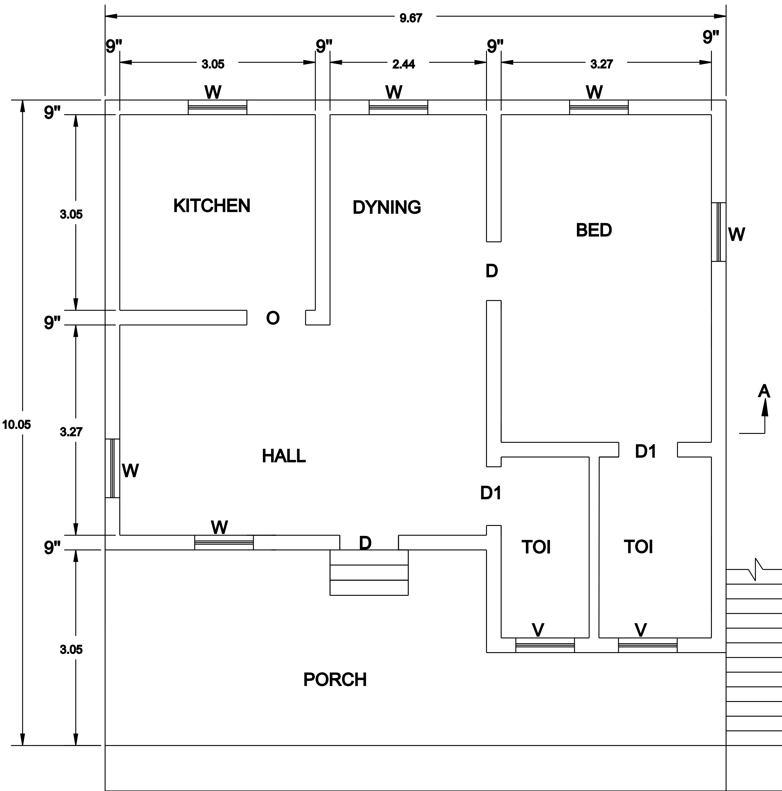
PROPOSED F.F PLAN
