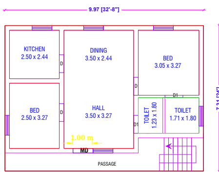
FIRST FLOOR PLAN [ NORTH FACING ]
