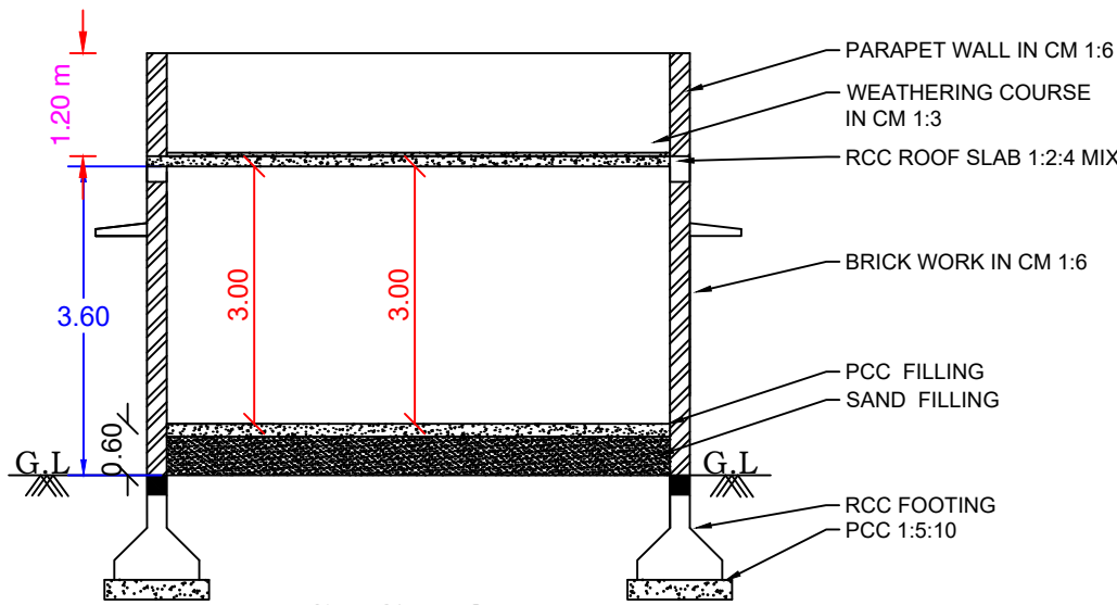
SECTION
