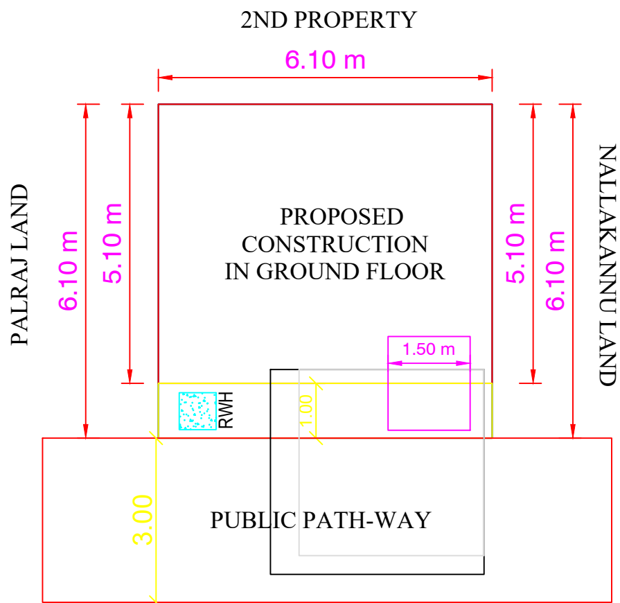
SITE PLAN
