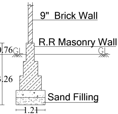
FOUNDATION DETAILS
