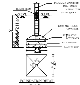
FOUNDATION DETAIL
