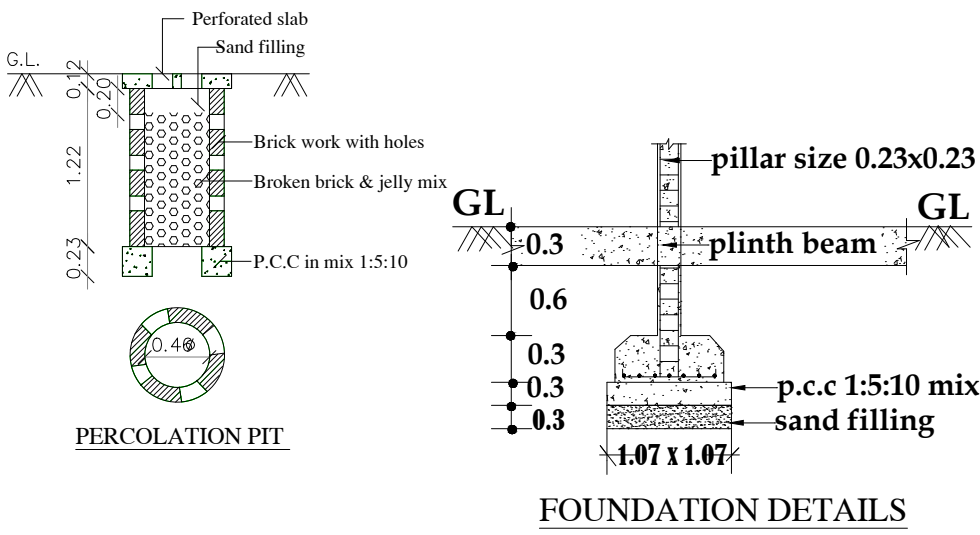
FOUNDATION DETAILS
