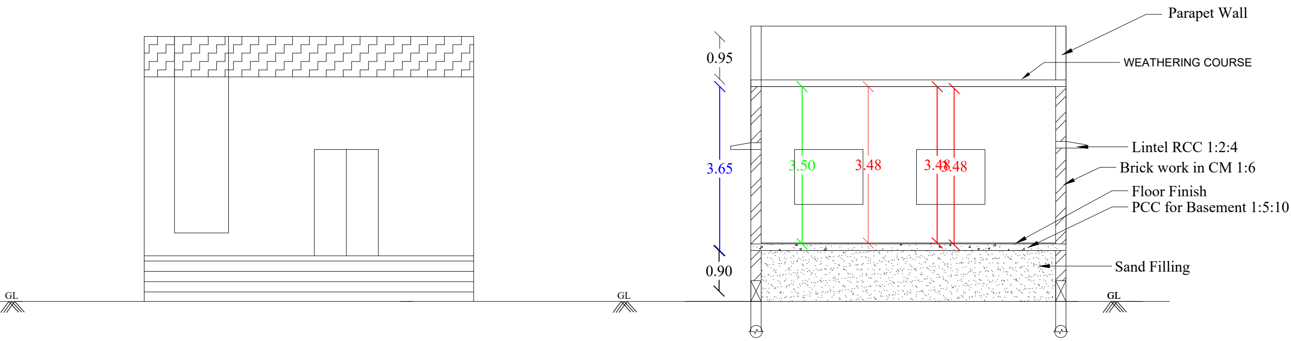
FRONT ELEVATION
