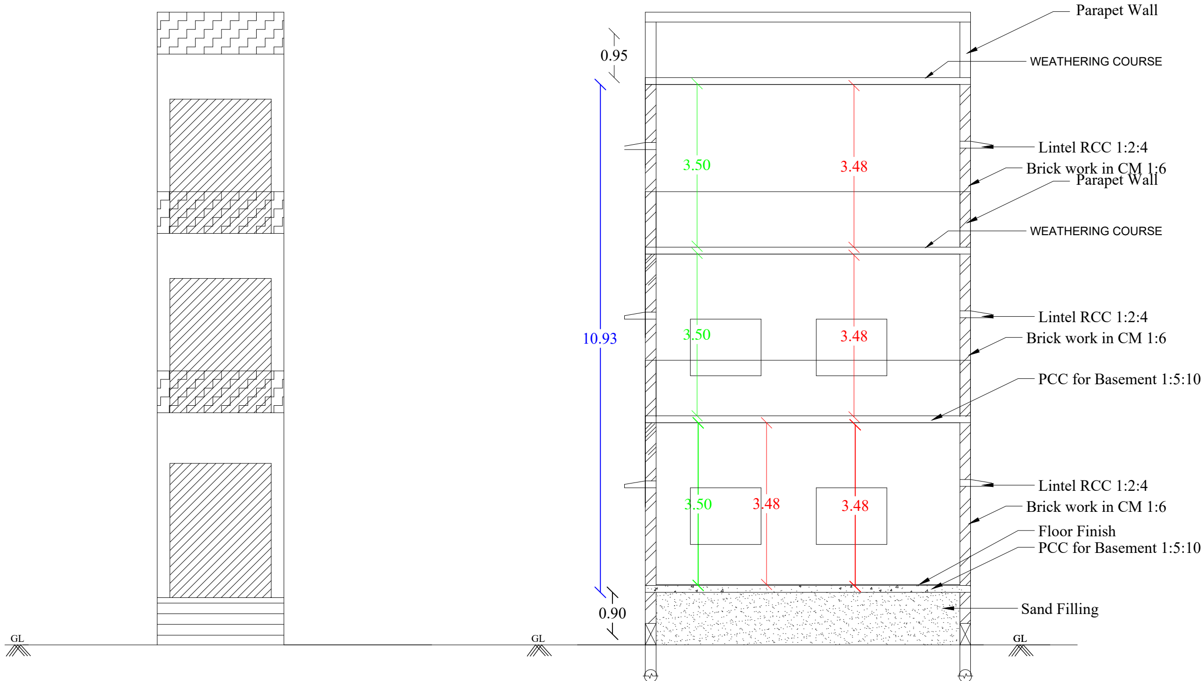
FRONT ELEVATION
