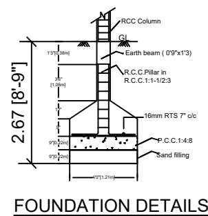
FOUNDATION DETAILS
