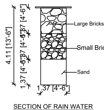
SECTION OF RAIN WATER
