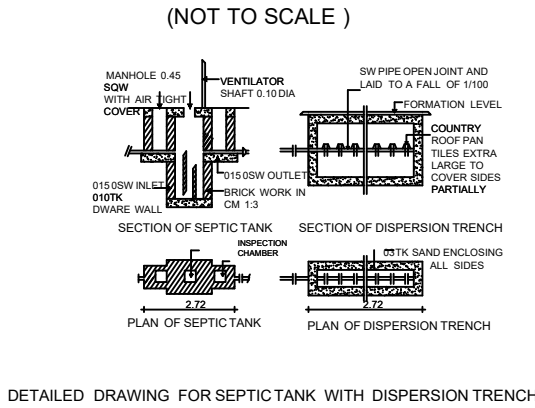
DETAILED DRAWING FOR SEPTIC TANK WITH DISPERSION TRENCH
