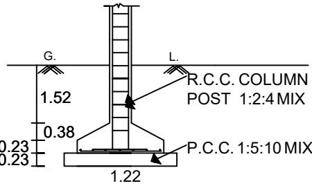
FOUNDATION DETAILS
