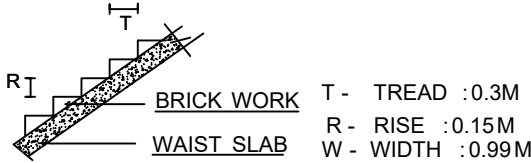
STAIRCASE DETAILS
