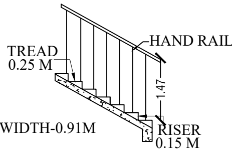
STAIRCASE DETAILS
