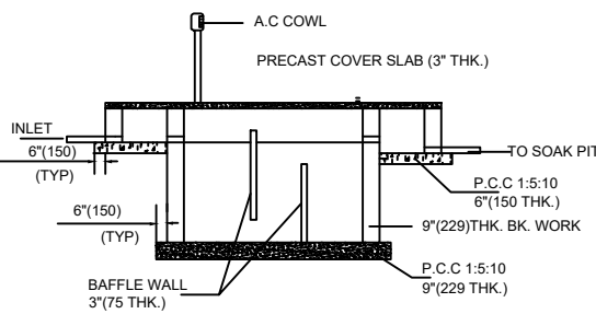
SECTION - BB PLAN OF SEPTIC TANK
