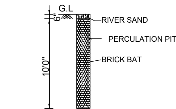
PERCULATION PIT
