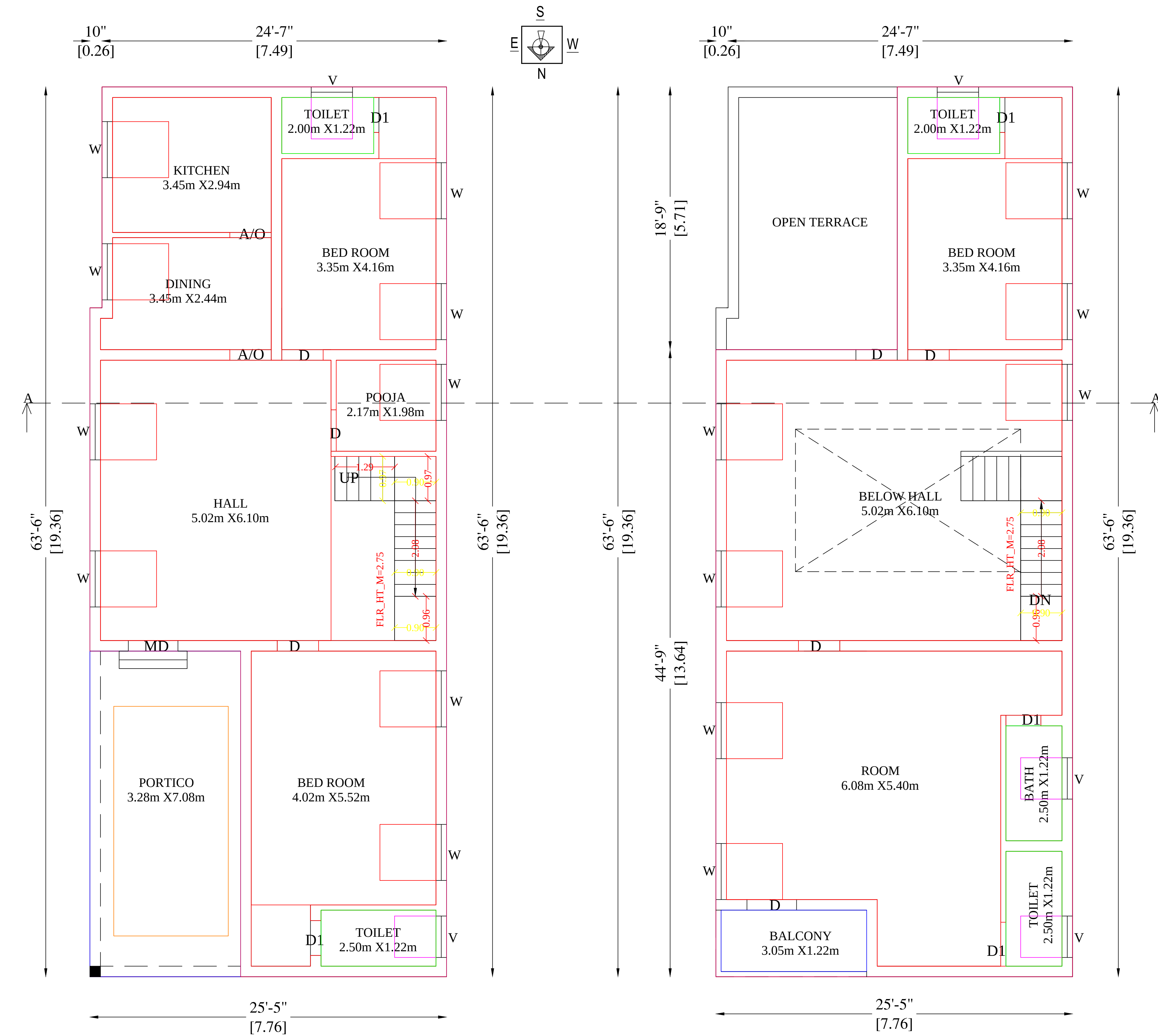
PRO.GROUND FLOOR PLAN
