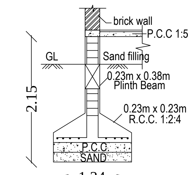
FOUNDATION DETAILS
