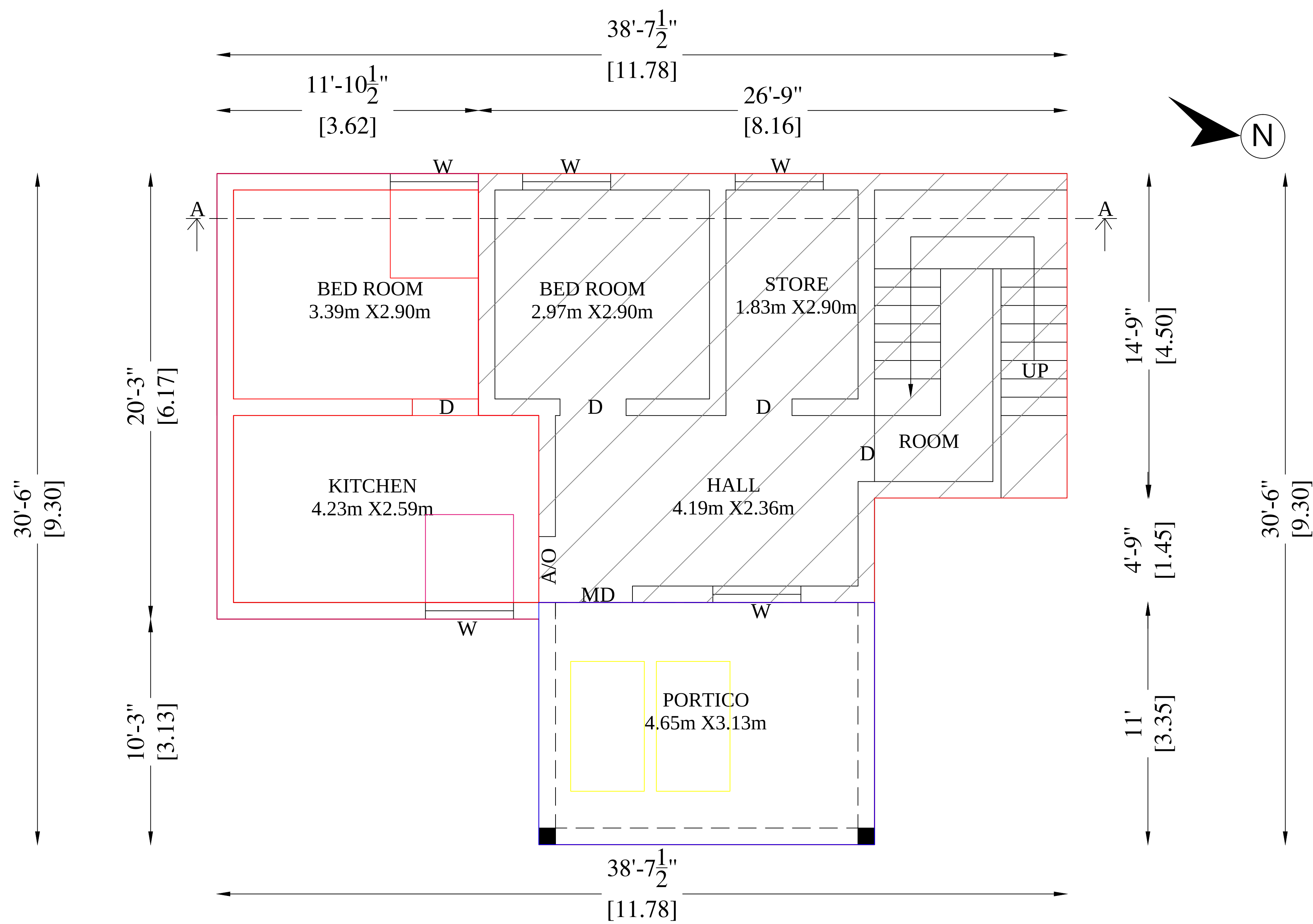
EXG. & PRO.GROUND FLOOR PLAN
