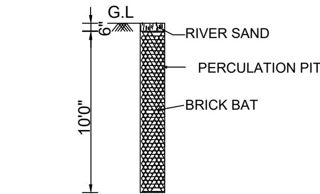
PERCOLATION PIT
