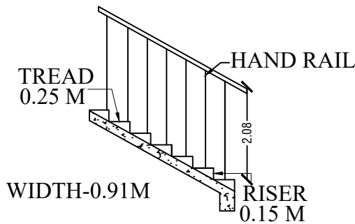
STAIRCASE DETAILS
