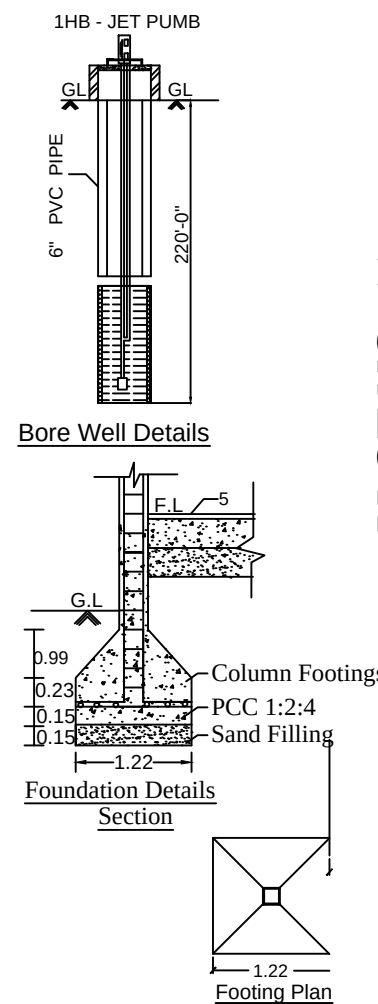
Footing Plan
