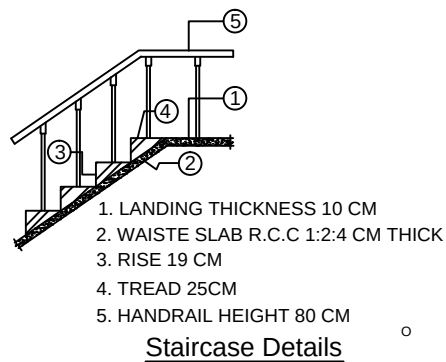
Staircase Details
