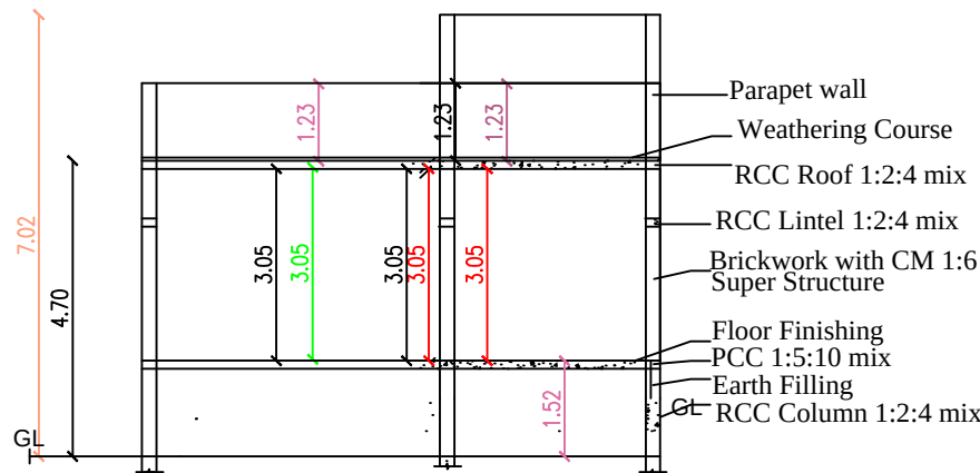
SECTION ON "VR"
