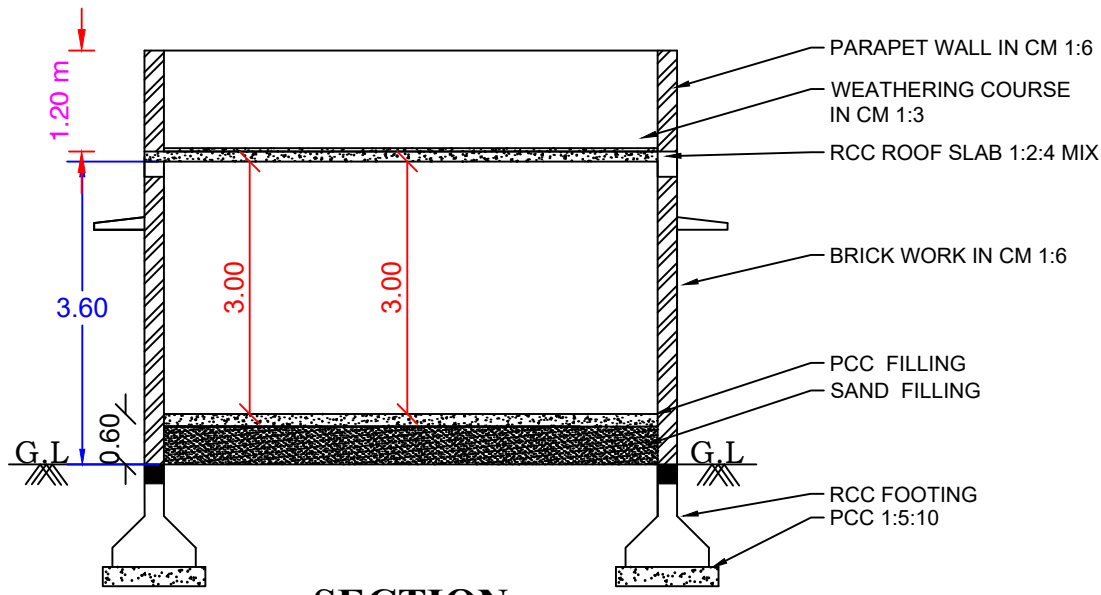
SECTION
