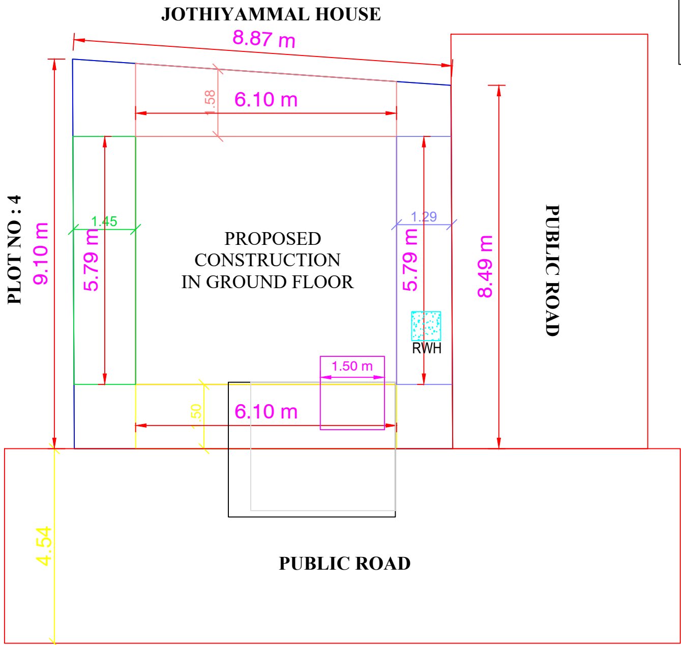
SITE PLAN
