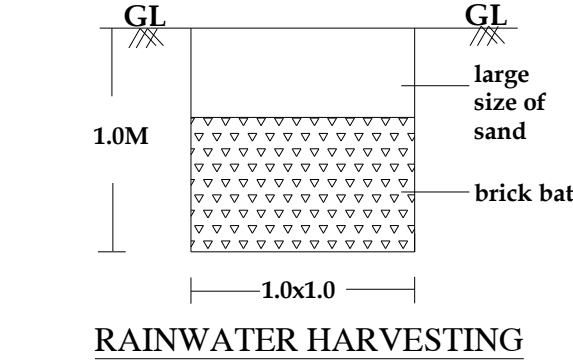
RAINWATER HARVESTING
