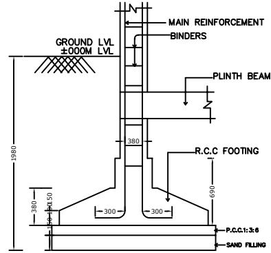
TYPICAL SECTION OF R.C.C COLUMN FOUNDATION SCALE : 1" = 2'-0"
