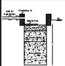
RAIN WATER PERCOLATION PIT
