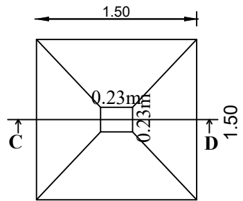
SECTION - 'CD'
