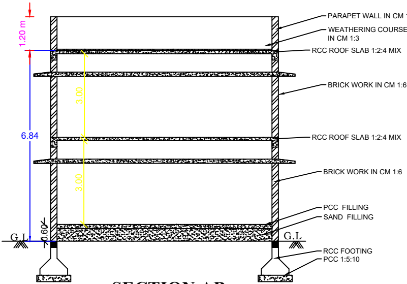
SECTION AB
