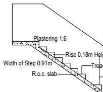
DETAILS OF STAIR CASE
