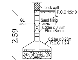
FOUNDATION DETAILS
