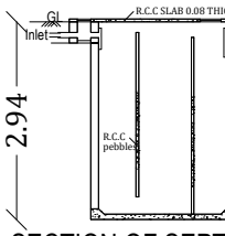
SECTION OF SEPTIC TANK
