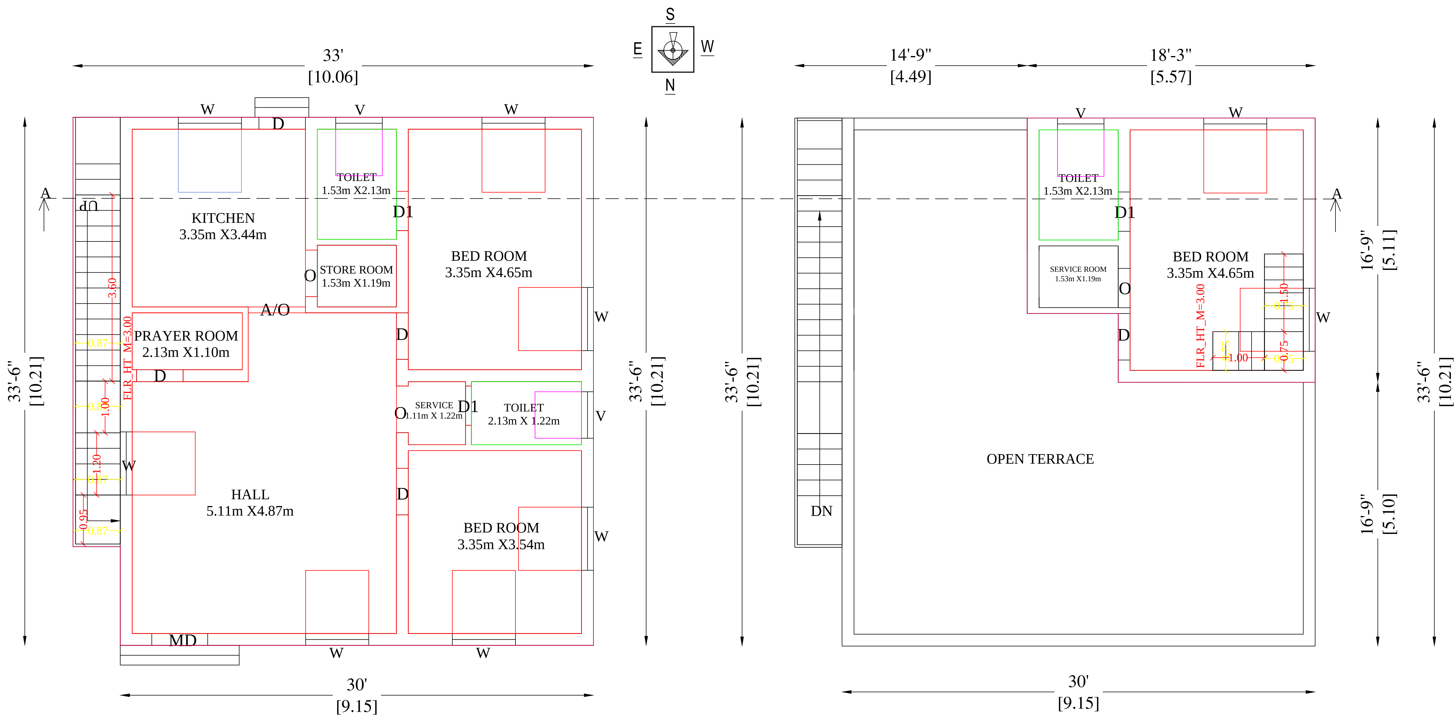
PRO GROUND FLOOR PLAN
