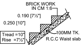
SECTION OF STAIR CASE (SCALE = 1:25)
