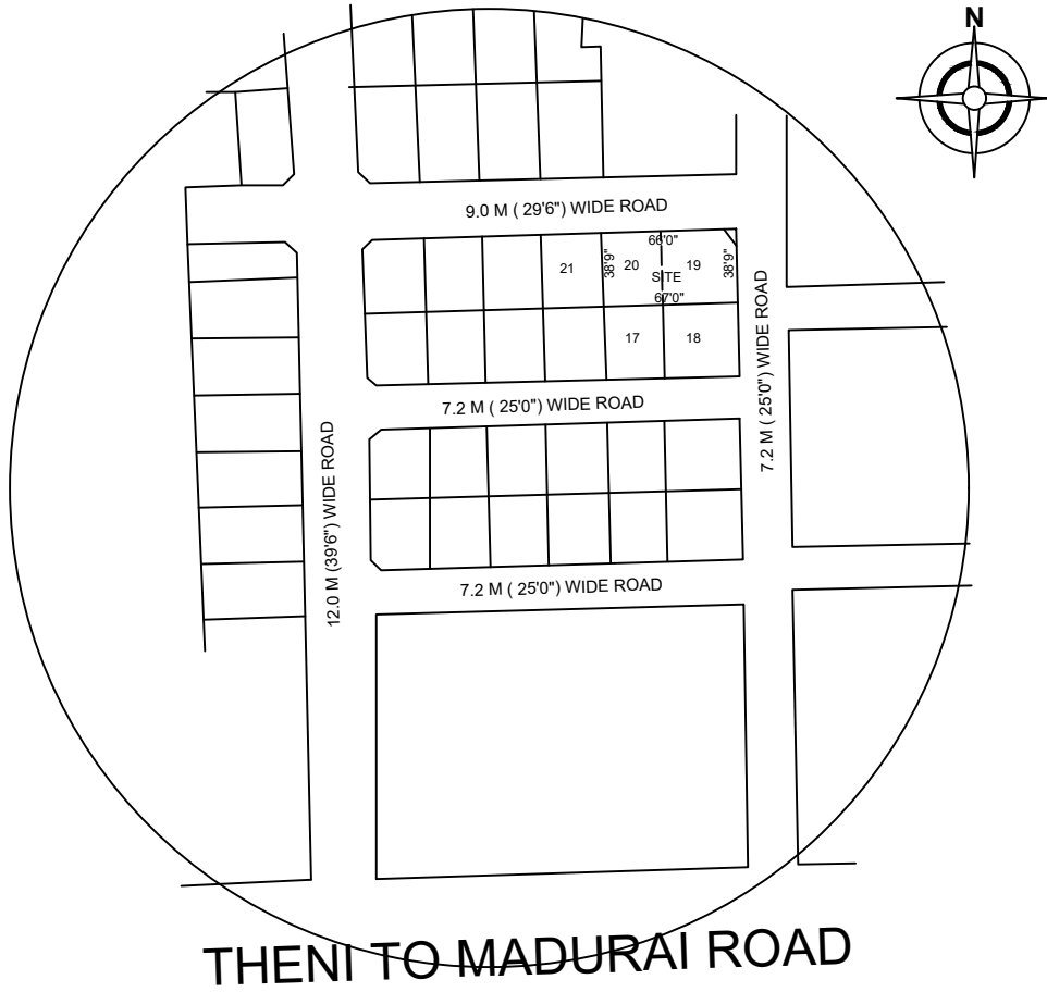
SITE PLAN KARADIPATTI VILLAGE
