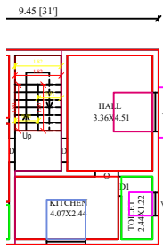
ST FLOOR PLAN
