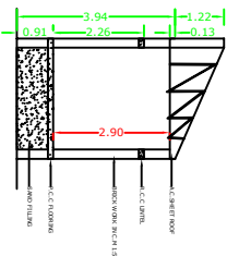
SECTION ON A-A
