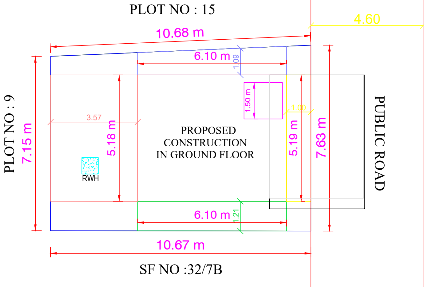
SITE PLAN
