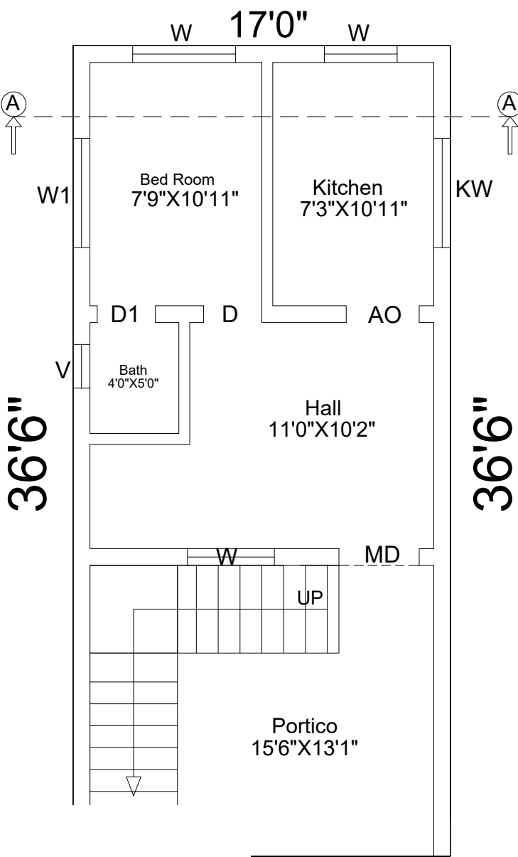
LOOR PLAN 7'0"
