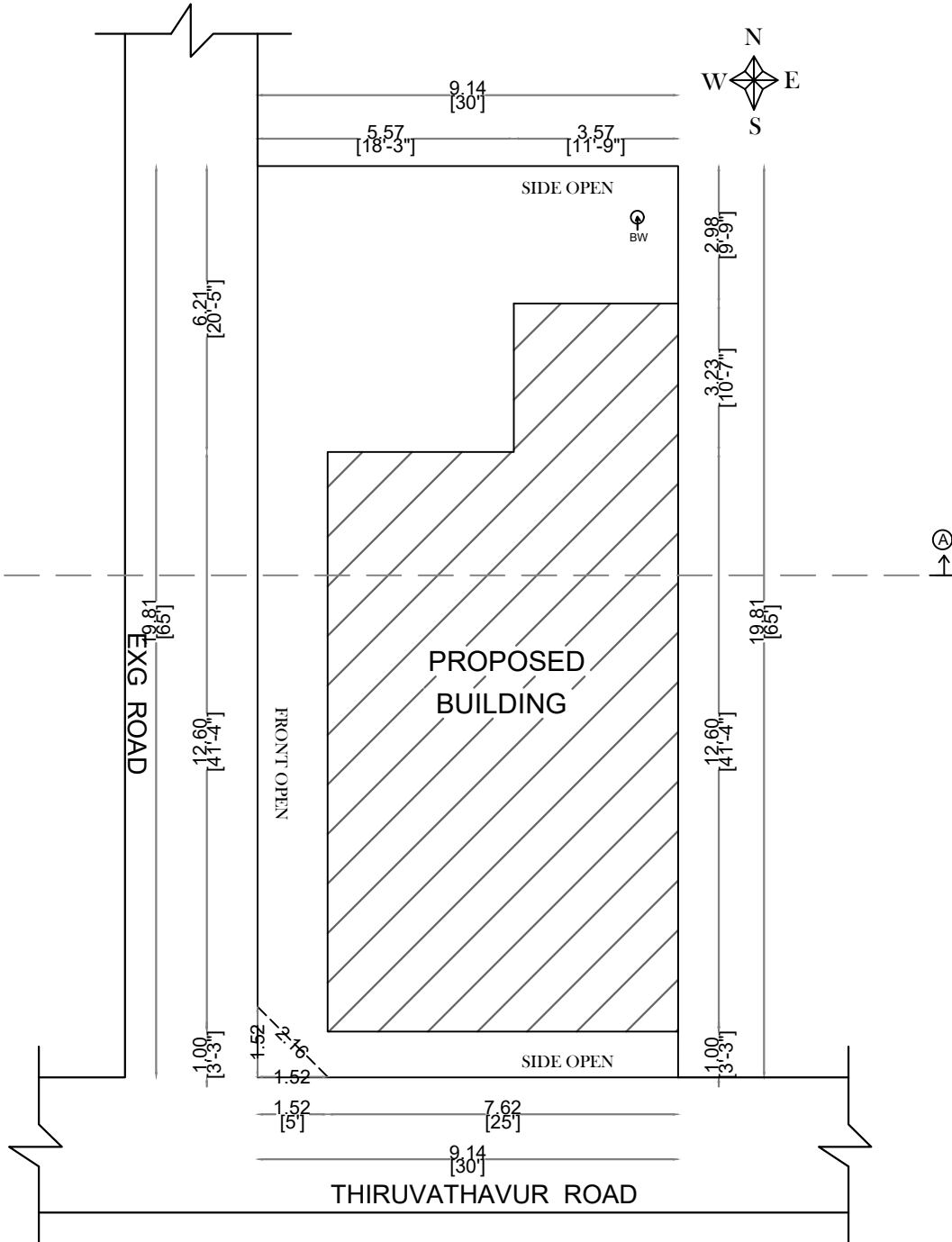
SITE PLAN
