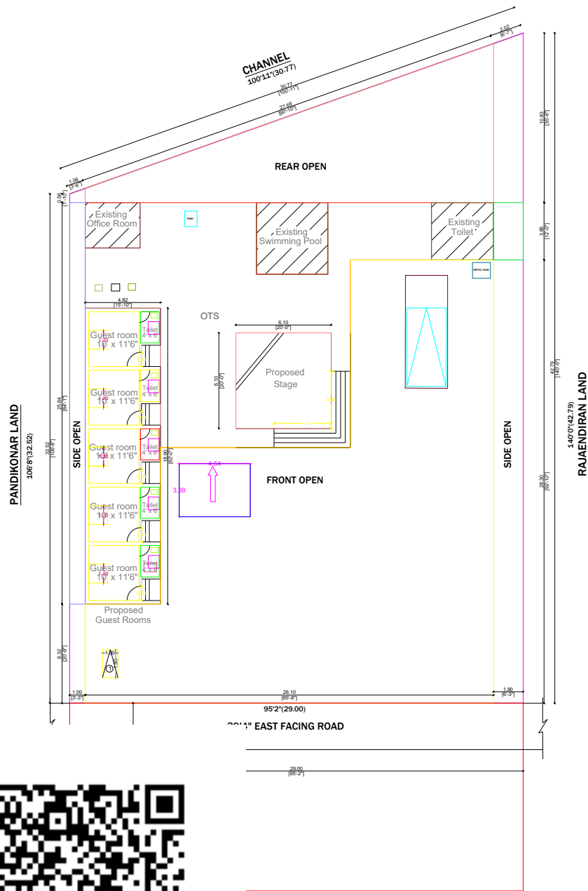
SED GROUND FLOOR PLAN
