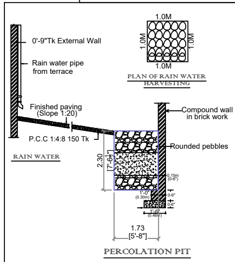
PLAN OF RAIN WATER HARVESTING
