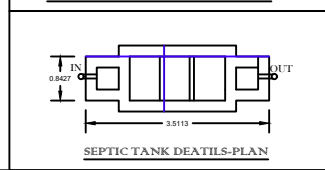
SEPTIC TANK DETAILS-PLAN
