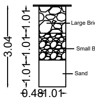
SECTION OF RAIN WATER COLLECTION PITS (NTS)
