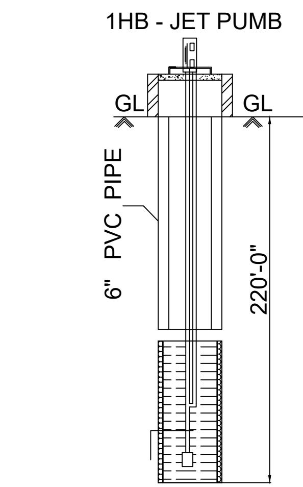
Bore Well Details
