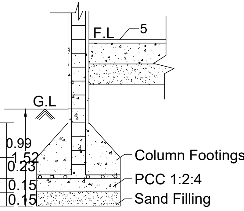
Foundation Details
