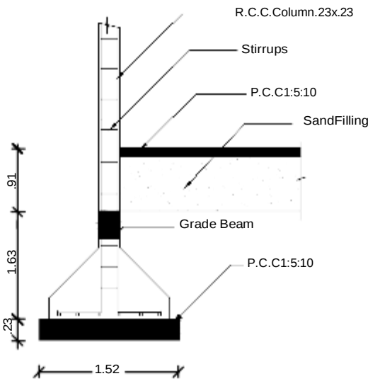
COLUMN DETAIL
