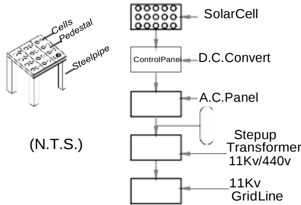
SOLAR SYSTEM FLOW DIAGRAM
