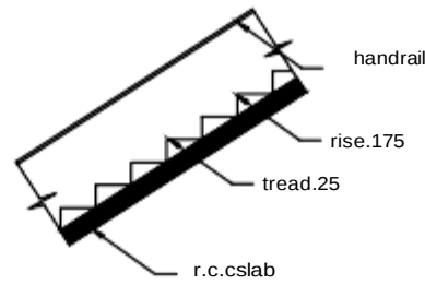
STAIR
