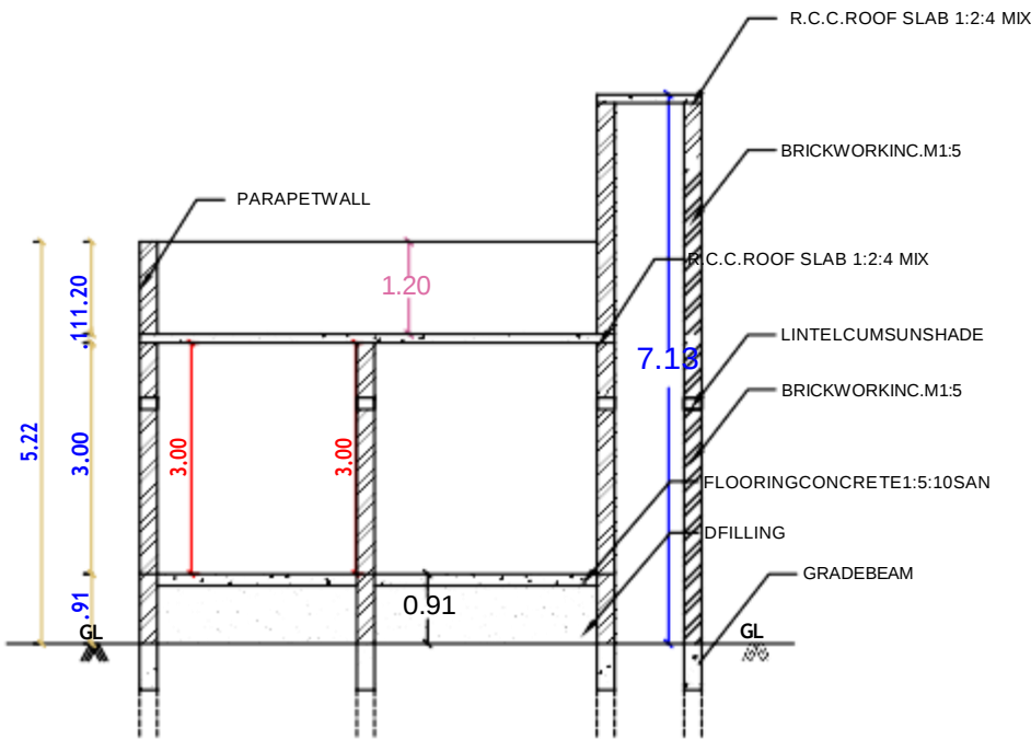
SECTION-AB
