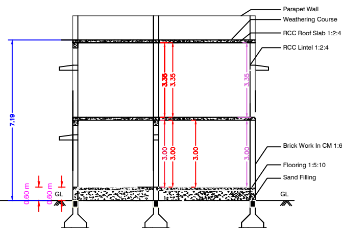
SECTION-AB
