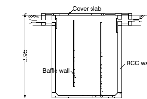
SECTION OF SEPTIC TANK
