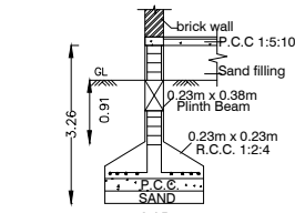
FOUNDATION DETAILS
