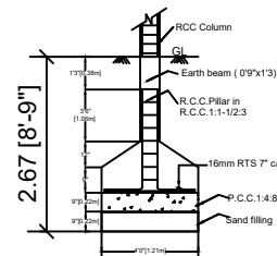
FOUNDATION DETAILS
