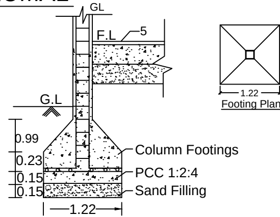
Foundation Details Section
