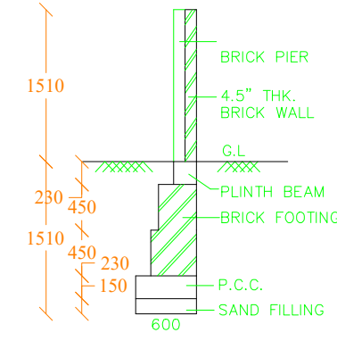
COMPOUND WALL DETAIL SCALE : 1" = 100'
