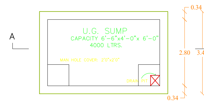
U.C. SUMP CAPACITY 6'-6" x 4'-0" x 6'-0" 4000 LTRS. SCALE 1" = 4' 0"
