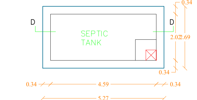
PLAN OF SEPTIC TANK SCALE 1" = 2'-0"
