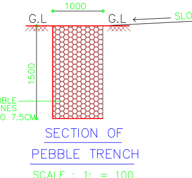
SECTION OF PEBBLE TRENCH SCALE : 1" = 100'
