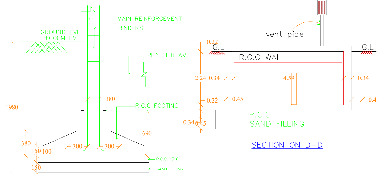
TYPICAL SECTION OF R.C.C. COLUMN FOUNDATION SCALE : 1" = 2'-0"
