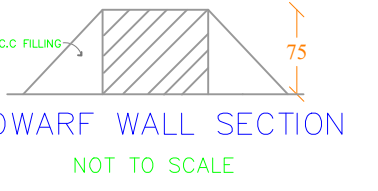
DWARF WALL SECTION NOT TO SCALE
