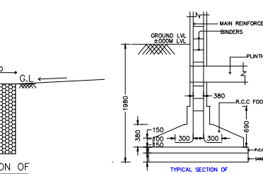
SECTION OF PEBBLE TRENCH SCALE : 1: = 100
