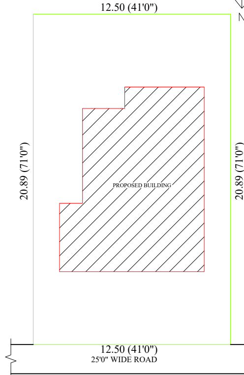
SITE PLAN
